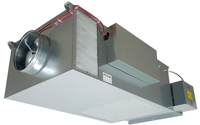
Type VFS-model 3, inlet 315mm
