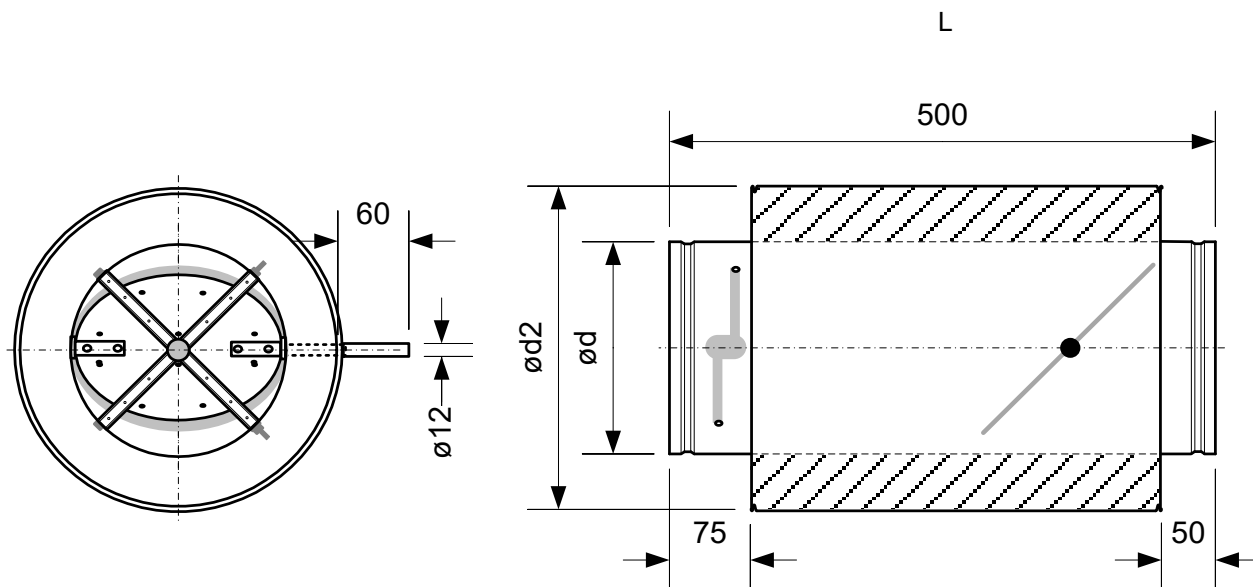
Type VSR-DW (double wall construction)
