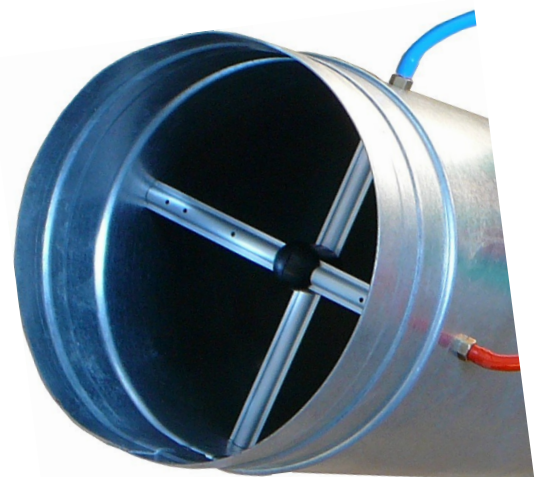
Detail FloXact-X® multipoint, averaging air flow sensor
