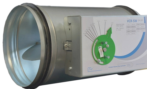
VCR-SW (single wall construction)
